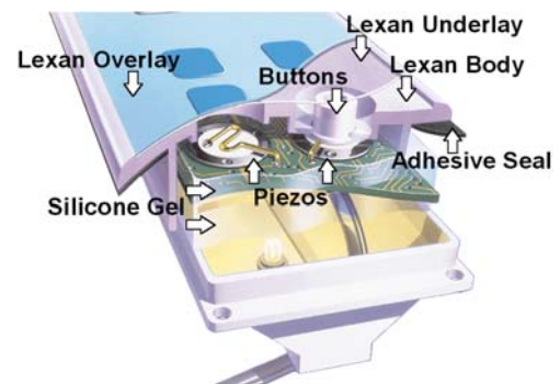
Panel Construction
