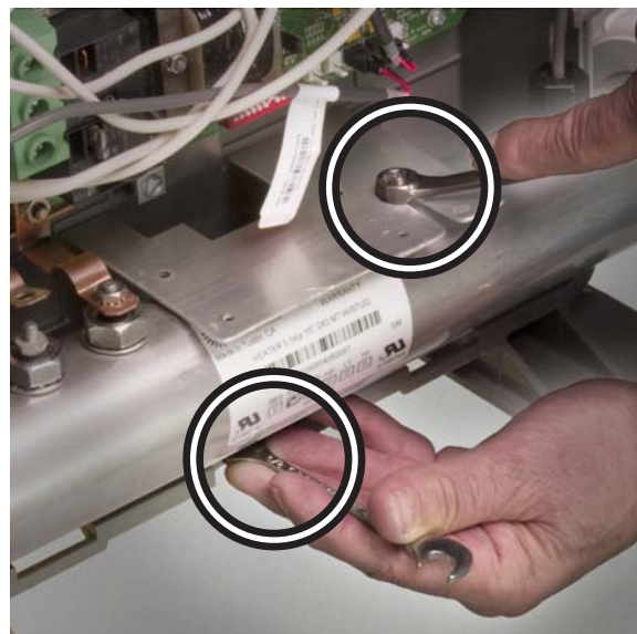
Remove both nuts that secure the element in place.
